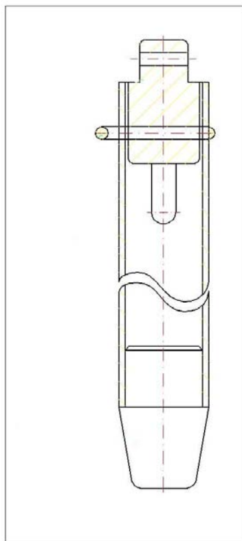
Bottom Nose for Link In TTG Link System
